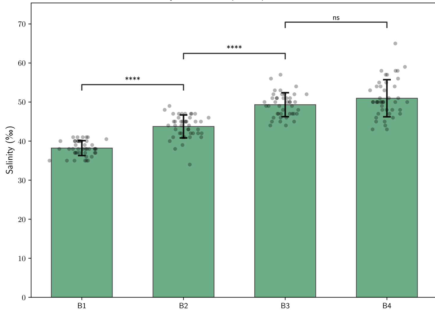
Mean salinity at 30 cm depth in piezometer at Babin
